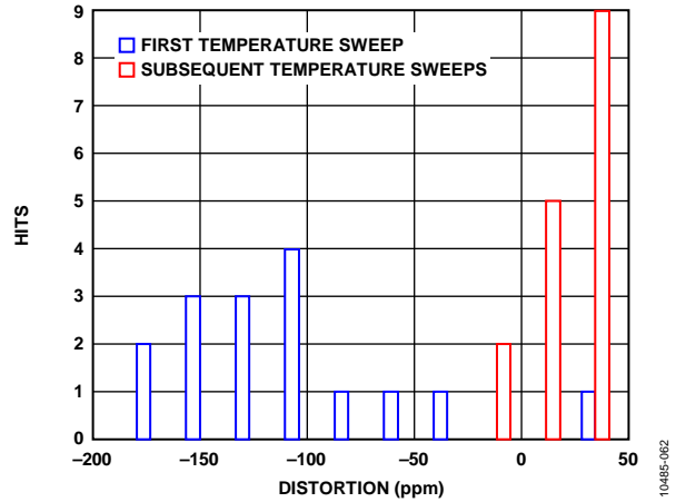
Figure 59. Thermal Hysteresis
