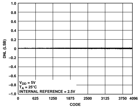
Figure 21. AD5684R DNL
