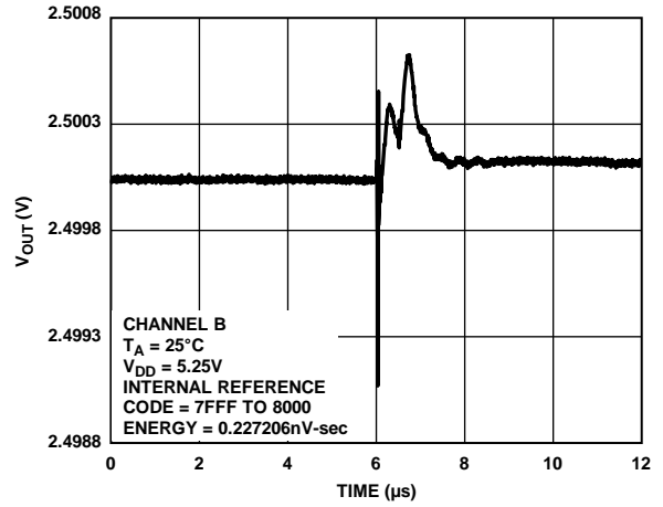
Figure 41. Digital-to-Analog Glitch Impulse
